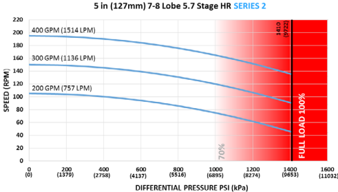
Speed Chart (See page 29)
