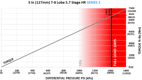
Torque Chart (See page 28)
