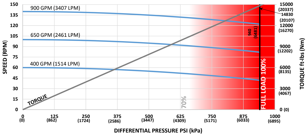
8 in (203mm) 7-8 Lobe 4.0 Stage HR
